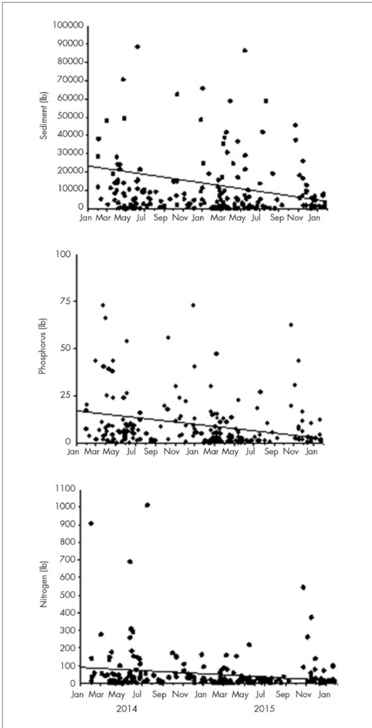
Figure 3. Sediment and nutrient loads leaving fields and running off into TWR systems annually (monitored for 2 years). Six TWR systems were monitored. The systems were within watersheds ranging from 141 to 385 acres and were all tilled land (except for turn rows). Solid lines represent the trend over the 2-year monitoring period.
